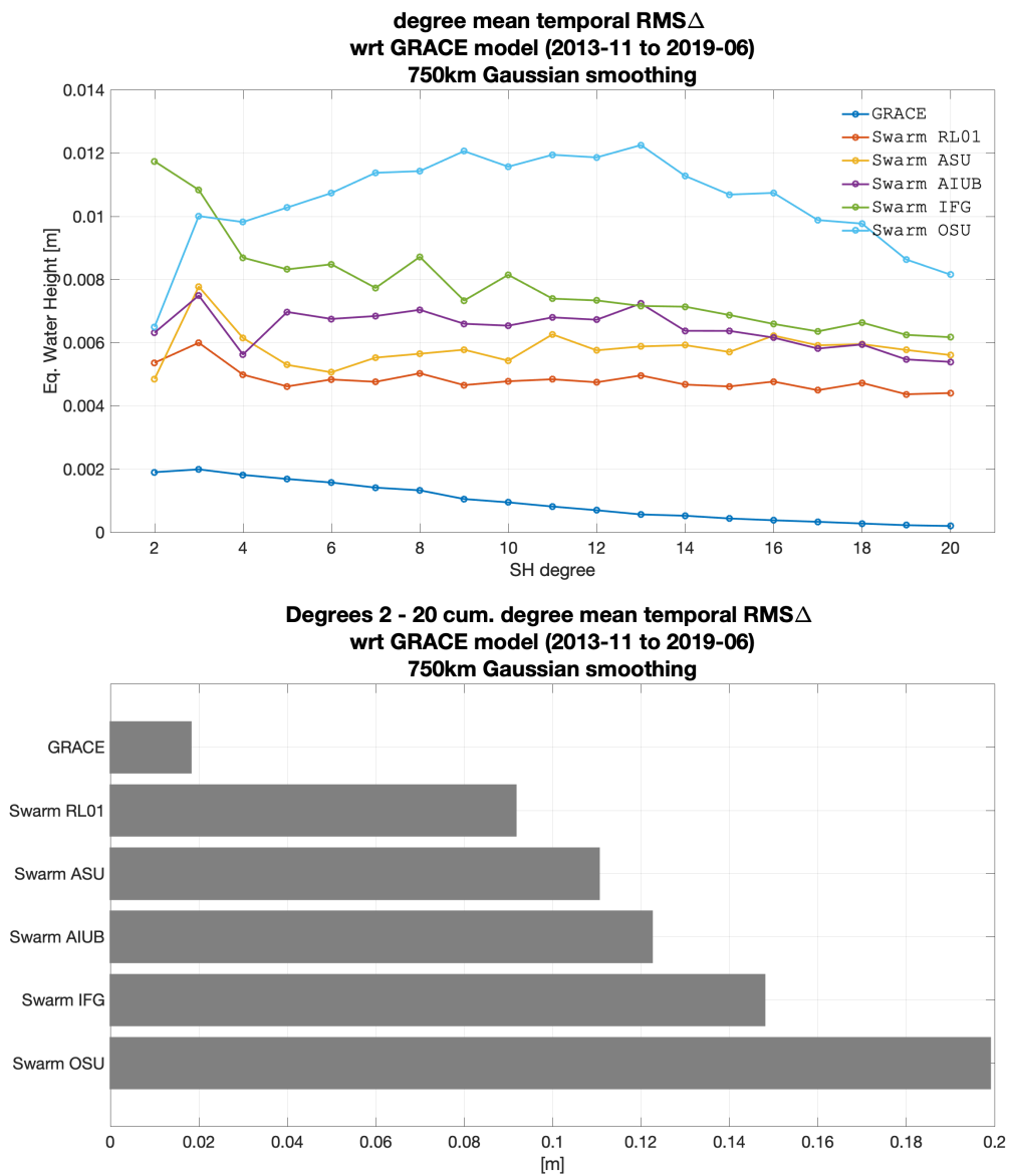
Figure 4 – Per-degree mean of the RMS difference (top) and cumulative degree-mean temporal RMS difference (bottom) between the Swarm GFMs and GRACE-based prediction, considering 750km Gaussian smoothing. This is (an estimate of) the average per-degree quality of the various Swarm solutions in the spectral domain (top) and globally (bottom) . The degree amplitudes remain relatively constant with increasing degree, instead of growing in terms of EWH, as the result of the smoothing.
