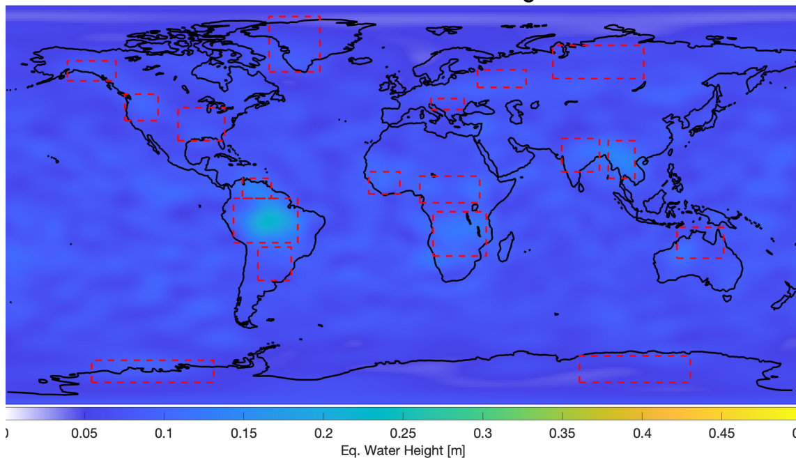
temporal STD of Swarm RL01 (2016-01 to 2019-09) 750km Gaussian smoothing
