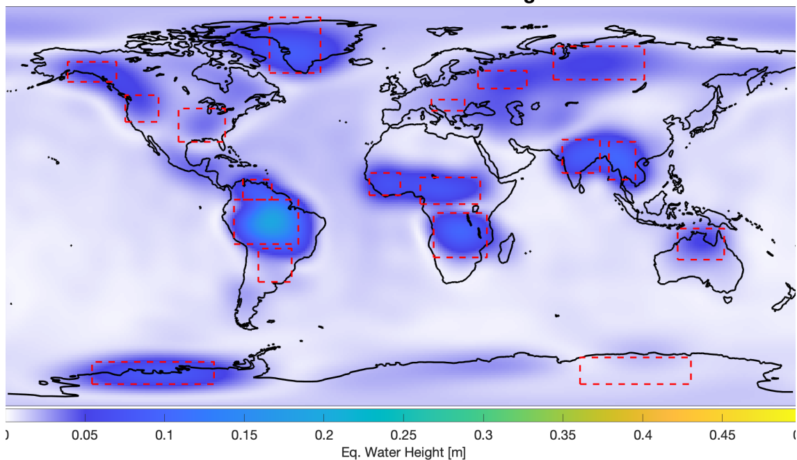
Figure 3 – Temporal variability of the GRACE/GRACE-FO climatological model, including the boundaries of the regions analysed in Section 5.3.1 to Section 5.3.18.
