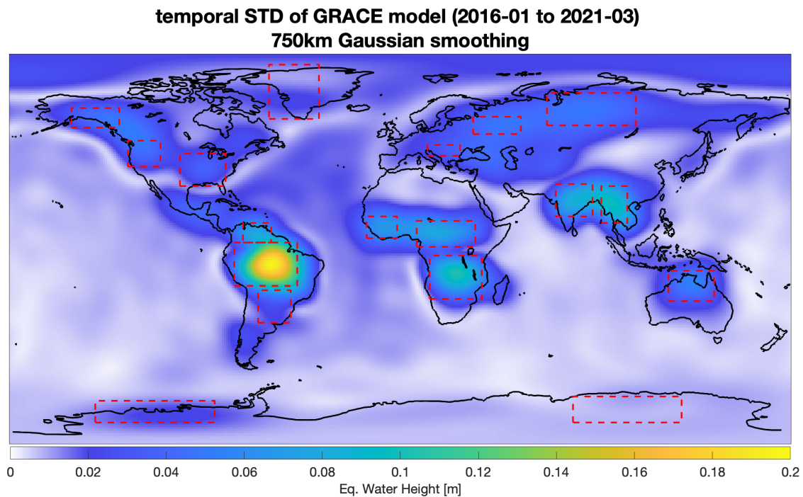
Figure 3 – Temporal variability of the GRACE/GRACE-FO climatological model, including the boundaries of the regions analysed in Section 5.5.1 to Section 5.5.18.
