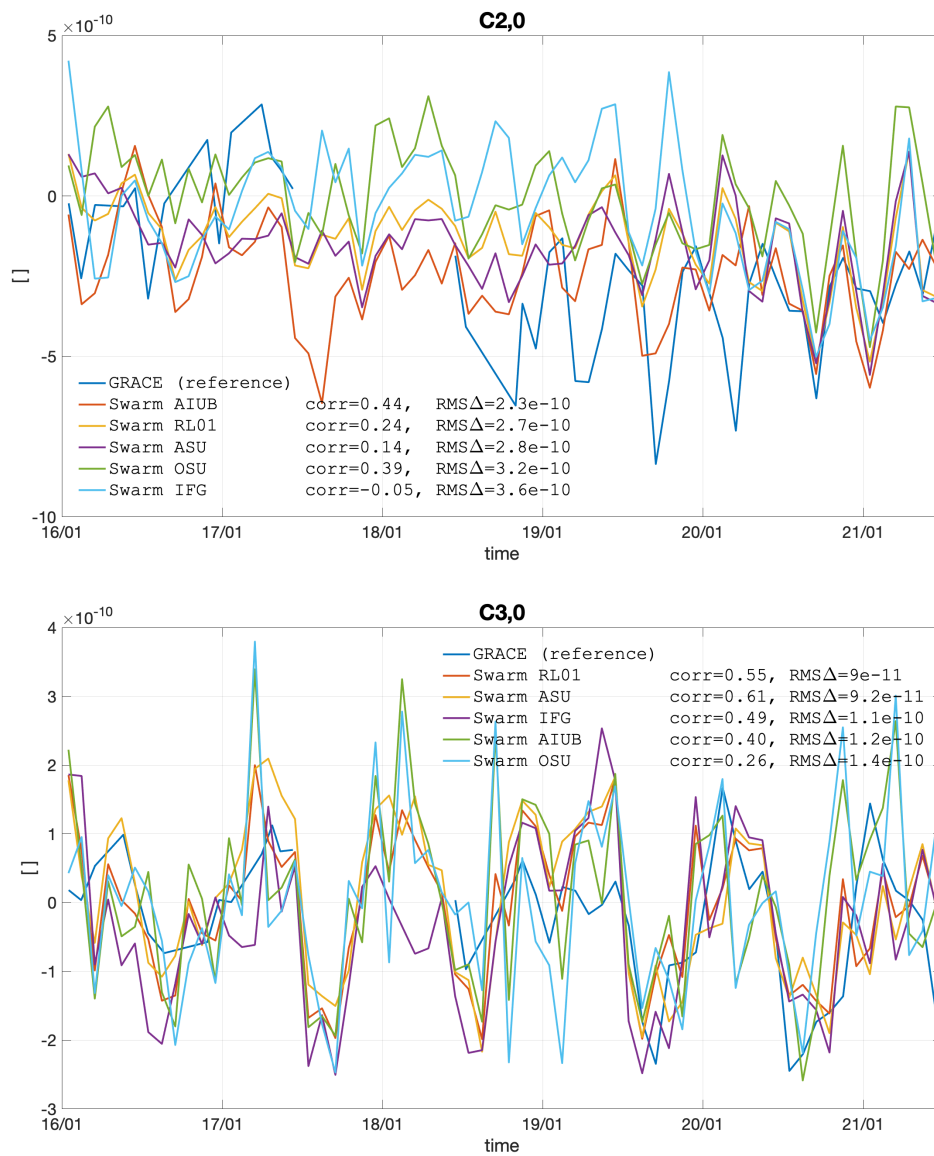
Figure 11 – Time series of the C_{20} (top) and C_{30} (bottom) coefficients, showing coefficients in the Swarm and GRACE/GRACE-FO GFMs, compared to Loomis and Rachlin (2020) (TN-14).
