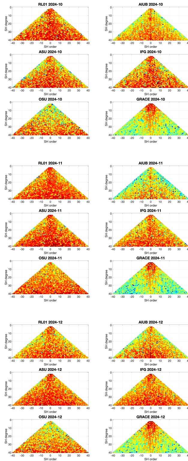
Figure 13 – Monthly triangular plots, all individual and combined Swarm solutions, as well as GRACE/GRACE-FO (no smoothing).
