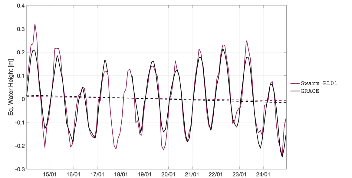
Figure 15 – Time series of EWH for the Amazon basin (latitude -17 to 3 degrees, longitude -76 to -47 degrees).
