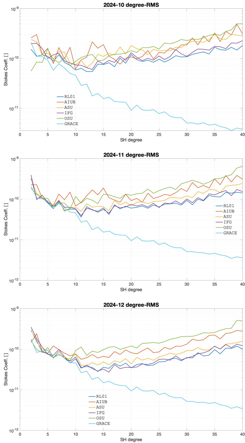
Figure 12 – Monthly degree-RMS, all individual and combined Swarm solutions, as well as GRACE/GRACE-FO (no smoothing).
