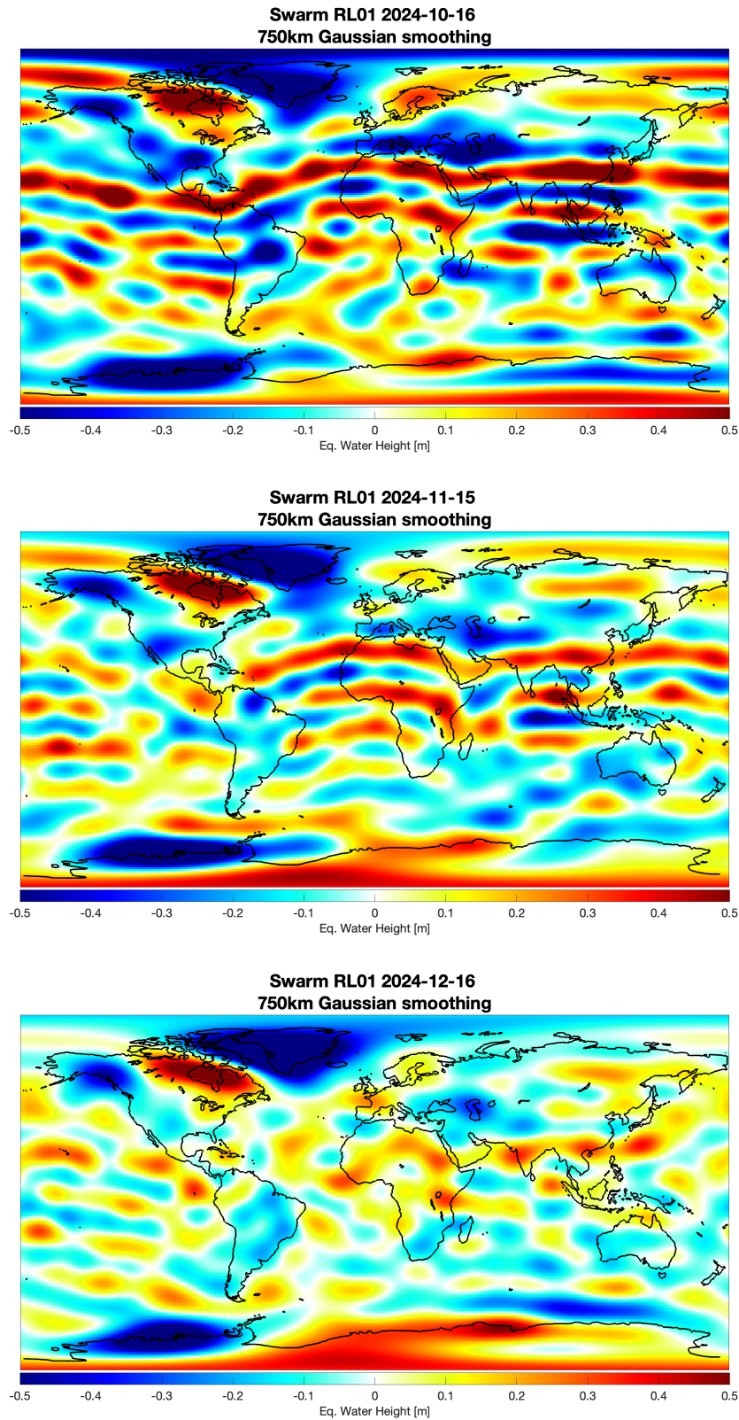
Figure 14 – Monthly maps for the combined Swarm solutions.
